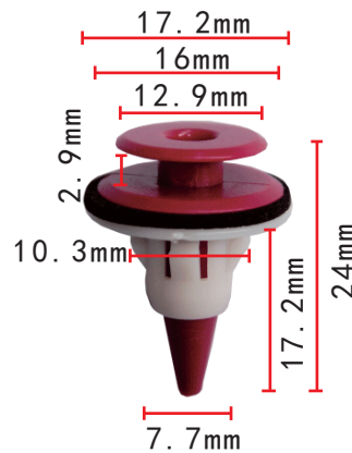
C1022 POM Mauve & White Trim Panel Retainer Nissan
