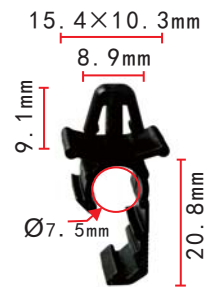
C1358 Nylon Black Pipe Retaining Clip
