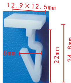
C1543 POM White Fender Retainer Toyota Lexus 52535-OEO030
