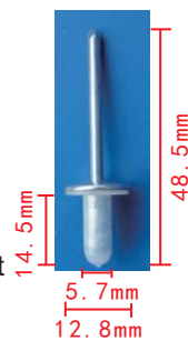
H2010 Valve Aluminum Rivet With Plastic Cap Toyota 90269-06013
