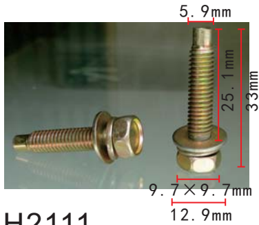
H2111 Zinc Color Screw
