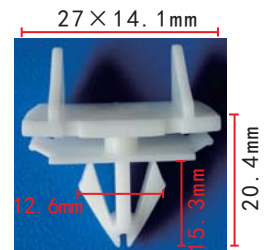
C1488 POM White Body Moulding Retainer BMW 51131829904
