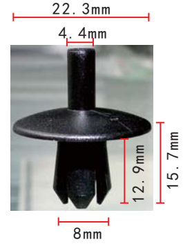
C1582 Nylon Black Push-Type Retainer Ford
