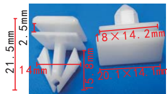
C1604 POM White Rocker Panel Retainer
