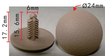
C1652 Nylon Coffee Roof Retainer European Car
