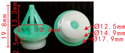
C1655 POM White & Green Trim Panel Retainer Land Rover 7703077354
