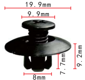
C1452 Nylon Black Push-Type Retainer Nissan 17575-0W010
