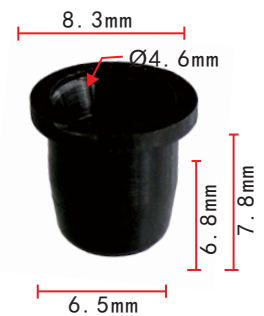
C464 Nylon Black Tubular Type Nut
