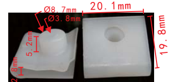
C1674 POM Original Body Pillar Retainer VW
