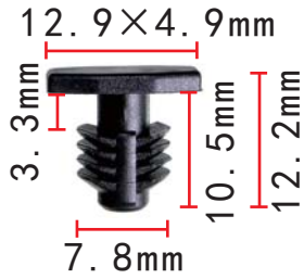
C3046 Nylon Black Front Cover Sealing Strip Retaining Clip Hyundai#86438-1R00
