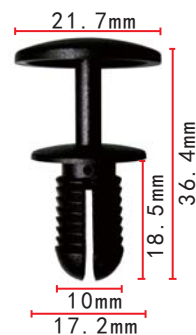
C1426 Nylon Black Push-Type Retainer VW, Audi
