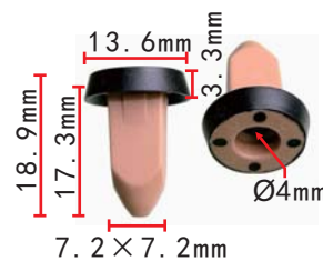
C3180 Nylon Brown(With Rubber) Rear Bumper Retaining Clip VW#N-105-073-01
