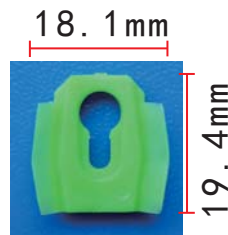
C408 Nylon Green Moulding Clip
