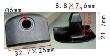
C1477 Nylon Black Rear Bumper Grommet Subaru 57750FC020
