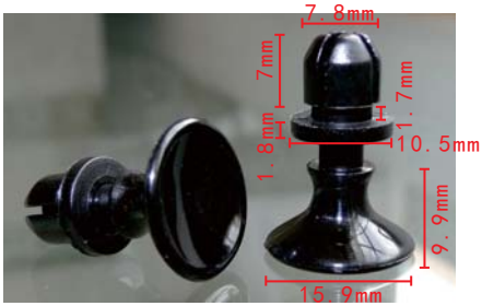
C1077 Nylon Black Push-Type Retainer
