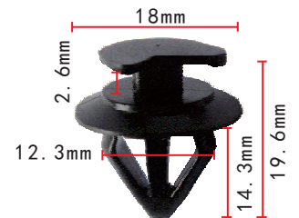
C989 POM Black Trim Panel Retainer BMW
