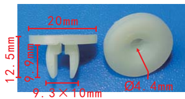
C3067 Nylon Light Green Mud Guard Panel Inner Retaining Clip Ford#6150260
