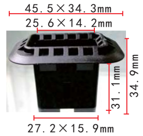
C1570 POM Black Back Seat Retainer VW Sagitar , MagotanB7L , Golf6 , CC , Passat , Lavida
