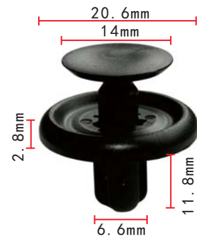
C999 POM Black Engine Under Cover Push-Type Retainer Toyota 90467-07201
