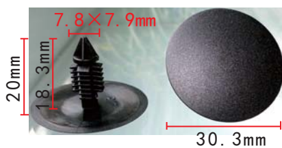
C1601 Nylon Black Retainer Land Rover
