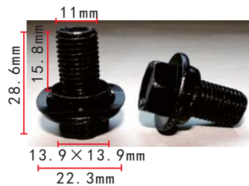
H2132 Zinc Black Bolt Toyota 90901-19040
