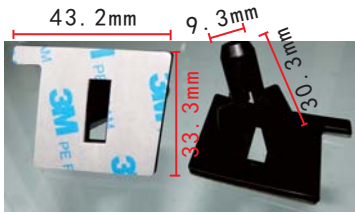
C1373 POM Black Windshield Retainer Square Bottom With 3M Adhesive Toyota Alphard
