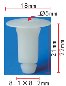
C976 Nylon Original Grommet Toyota
