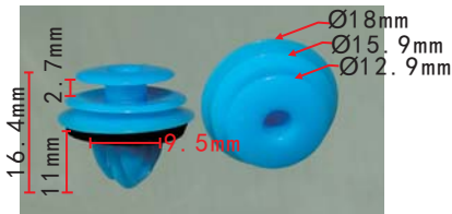
C1935 POM Blue Front Door & Back Door Trim Panel Retaining Clip Toyota#67771-26240
