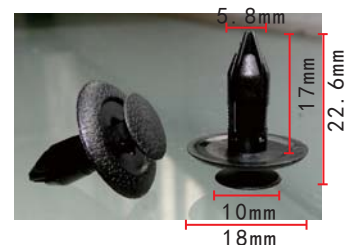
C1547 POM Black Trunk Top Ceiling Retainer Mazda B467-68-AC3 28 B467-68-AC3 25
