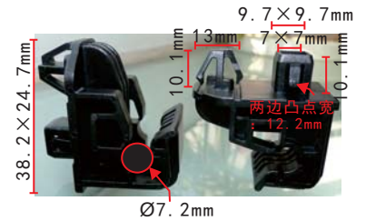
C1546 POM Black Front Head Lamp Bracket Retainer Nissan
