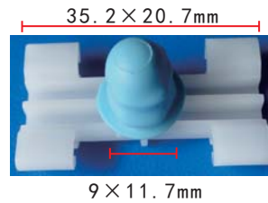
C1483 POM White & Blue Shield Door Trim Panel Clip BMW
