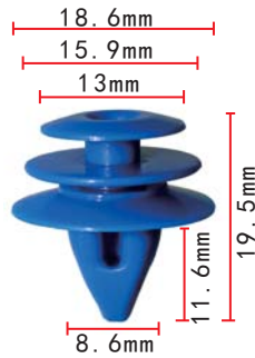
C1378 POM Blue Trim Panel Retainer Nissan
