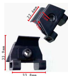
C3162 POM Grey Black Front Wheel Fender Retainer Toyota#53879-06100
