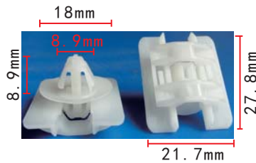
C1256 POM White Retainer
