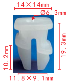
C1529 Nylon White Screw Seat Nissan 01281-00431
