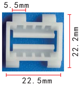
C978 POM White Retainer Mercedes-Benz A0019885081
