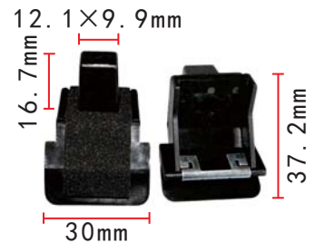
C1278 Nylon Black Retaining Clip Nissan
