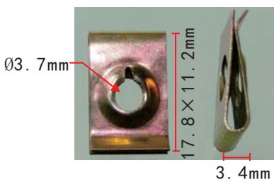
H2102 Zinc Color U-Type Iron Clip
