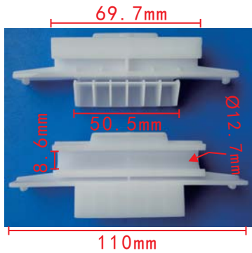
C1492 POM White Bumper Retainer Toyota Lexus Toyota Estima MCV40 2000-2003 On
