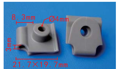
C1977 Nylon Grey Front Bumper U-Type Nut Mazda#C274-50-133
