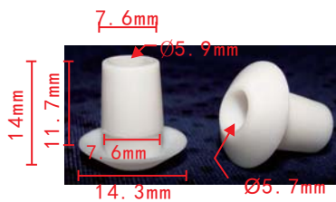
C1588 Nylon Milk White Trim Panel Base Rubber Shield Land Rover
