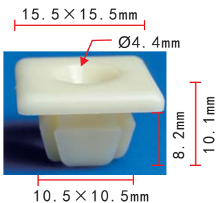
C29 Nylon White Front End & Instrument Panel Nut #8 Screw Size GM 3893980
