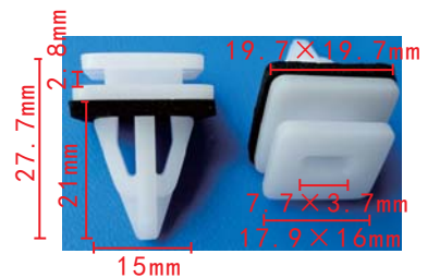
C1523 POM White Door Anti-Collision Strip Retainer Honda 90501-S9A-003
