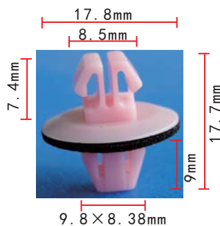
C378 POM White Rocker Panel Moulding Clip Toyota 90467-11063 Previa 1990-On
