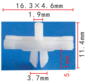
C252 POM White Body Side Moulding Clip Volvo 591740, 591-740
