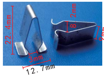
H2153 Zinc Clear Iron Clip
