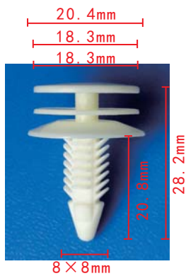
C637 Nylon Beige Door Trim Panel Retainer GM 15986673
