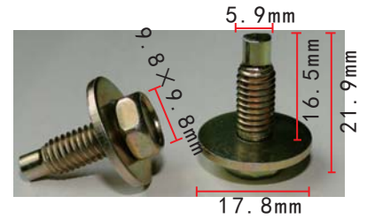
H2107 Zinc Color Screw
