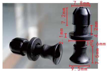
C1083 Nylon Black Push-Type Retainer
