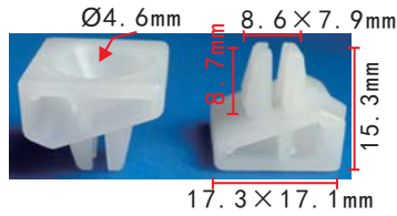
C1471 Nylon Original Screw Seat Subaru 94079AA000
