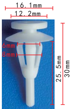
C819 POM White Door Moulding Retainer Chrysler M566719, MB566719
