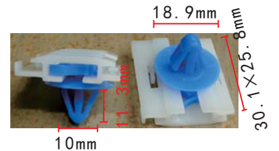
C1258 POM White & Blue Retainer
