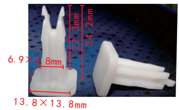
C1595 POM White Retainer Toyota RAV 4
