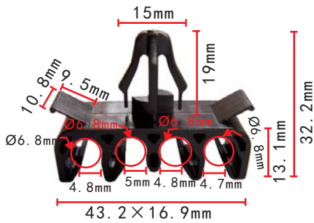
C1018 POM Black Routing Clip Toyota Hiace
