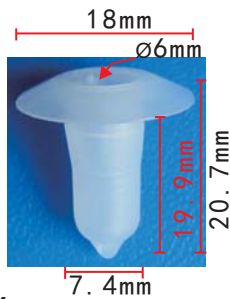
C1304 Nylon Original Retainer European Car
