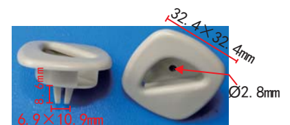
C1490 POM Light Grey Roof Insulation Cotton Retainer
