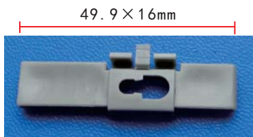
C432 POM Grey Moulding Clip
