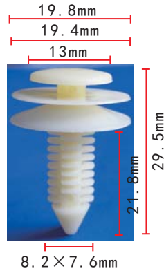
C172 Nylon White Trim Panel Retainer Ford 389144-S
