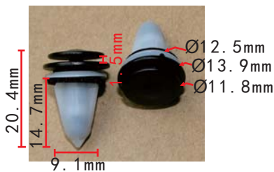
C3213 POM White & Nylon Black Trim Panel Retaining Clip
