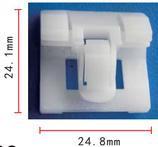
C62 POM White Belt Moulding Clip
