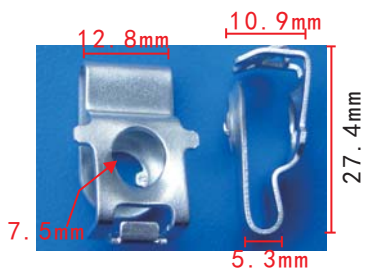
H2089 Zinc Clear Cross Recessed Screw Seat / Screw Retainer Audi
