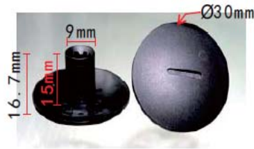
C1842 Nylon Black Wheel Housing / Door Trim Panel Retaining Clip Renault 7703081054
