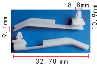
C1202 POM White G3 Routing Clip BYD
