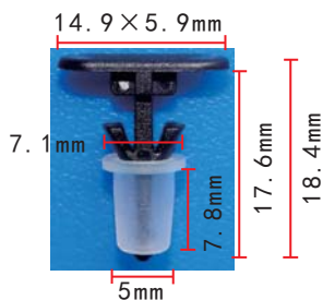
C921 Nylon Black Retainer VW
