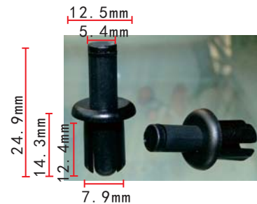
C1660 Nylon Black A Pillar Outer Trim Panel Retainer Land Rover
