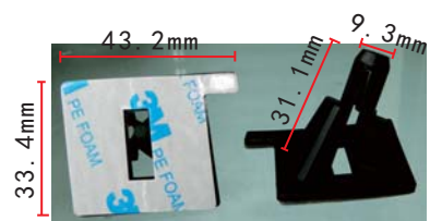
C1372 POM Black Windshield Retainer Square Bottom With 3M Adhesive Toyota Alphard
