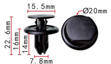
C1981 POM Black Radiator Grille/ Air Filter Retaining Clip Mazda#BGV4-56-145
