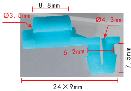
C494 Nylon Blue Rod End Clip-Right Holds 4mm Prop Rod Mazda 9927-80-404 Ford E6DZ5421952A, E83Z-5421952B
