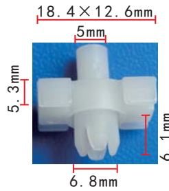
C934 Nylon White Body Side Retainer
