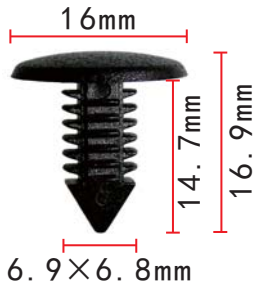
C1349 Nylon Black Trim Panel Retainer
