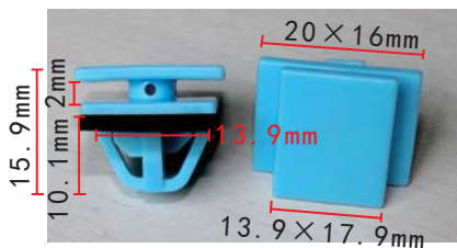
C1961 POM Light Blue Rocker Panel Sill Fender Clip Hyundai#87756-D3000
