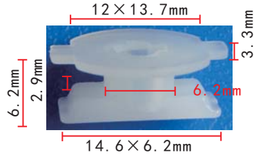
C982 Nylon Original Side Rocker Panel Clip Hyundai 87719-3D000
