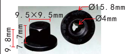
C1759 Nylon Black Wheel Cover Nut GM, Ford&Opel 90413589,180942
