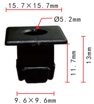
C457 Nylon Black #12 Screw Size Chrysler 6032516
