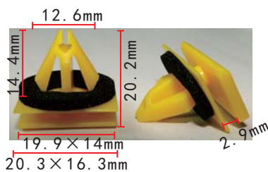
C1540 POM Yellow Rocker Panel Retainer GM 5480852
