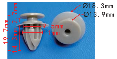
C1982 POM Grey Fender Flare Moulding Clip Mazda#KD53-51-W24
