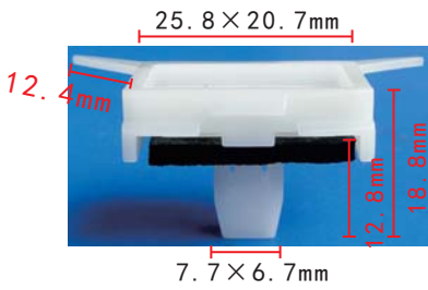
C820 POM White Windshield Clip Acura 91537-SP0-013 Legend 1991-On
