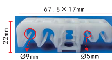
C1206 POM White Routing Clip Toyota Alphaard
