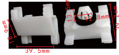
C1654 POM White Door Anti-Collision Retainer Land Rover DYC000091
