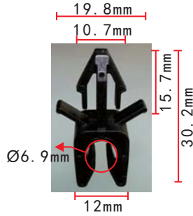
C1377 Nylon Black Pipe Clip
