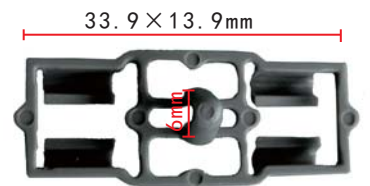
C965 Nylon Grey Retaining Clip
