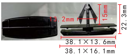
C1625 POM Black Rocker Panel Retainer
