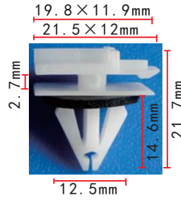
C958 POM White Moulding Clip
