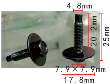
H2112 Zinc Black Screw
