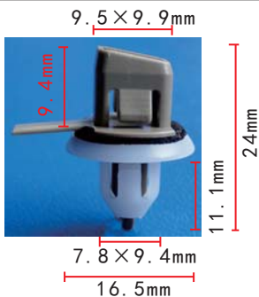
C226 POM Brown & White Door Lower Moulding Clip
