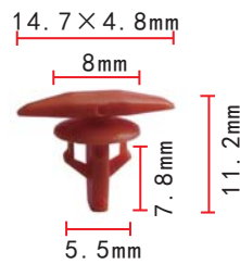
C66 Nylon Orange Weatherstrip Retainer Honda 91530-SP1-003
