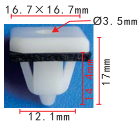
C970 POM White Nylon Nut With Sealer Hyundai 87758-37000
