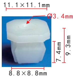
C29 Nylon White Front End & Instrument Panel Nut #8 Screw Size GM 3893980
