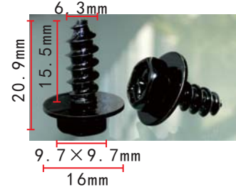
H2135 Zinc Black Screw Toyota 90159-C0036
