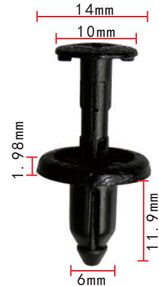
C997 POM Black Vent Cover Push-Type Retainer Toyota Hiace
