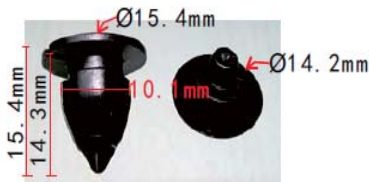
C1819 POM Black Trim Panel Retaining Clip Renault 7703077434
