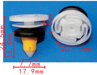
C3203 POM Yellow White(With Rubber) Front Door & Rear Door Trim Panel Clip
