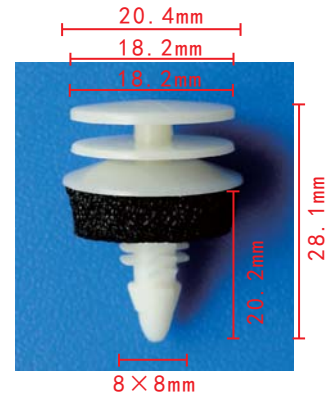
C646 Nylon Beige Trim Panel Retainer With Sealer GM 22646099
