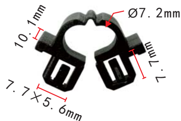
C1368 Nylon Black Guider Clip
