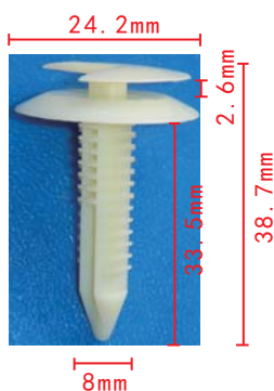
C38 Nylon Beige Trim Panel Retainer GM 1987-On 10126901
