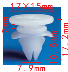
C3087(TF57) POM White Body Anti-Collision Fender Clip Volvo#30784514
