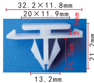
C1519 POM White Door Moulding Clip GM
