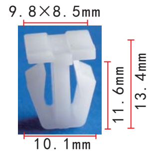
C112 POM White Body Side Moulding Clip
