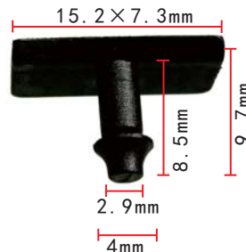
C1473 Nylon Black Retainer Honda 91590-SV4-003
