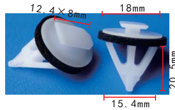
C1614 POM White Rocker Panel Retainer Honda 75315-S9A-004
