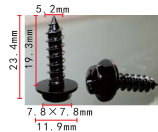
H2136 Zinc Black Screw Toyota 75392-42030
