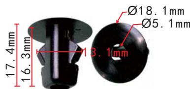
C3008 Wheel Arch Fender Grommet Citroen#6822QP
