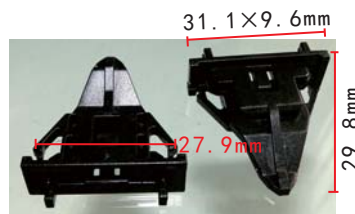
C1754 POM Black Front Fender Inner Lining Retaining Clip Toyota 61991-35010
