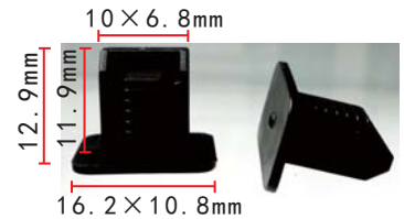
C1571 Nylon Black Rear Windshield Top / Top Ceiling / D Pillar Retainer VW Jetta 357-867-646 ; Audi
