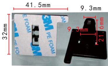
C1375 POM Black Windshield Retainer Square Bottom With 3M Adhesive Toyota Alphard
