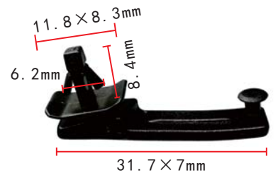
C1383 Nylon Black Front Door Weatherstrip Retainer Honda Accord
