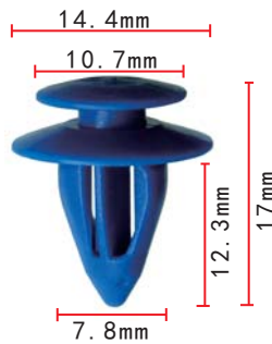
C1379 POM Blue Trim Panel Retainer Mitsubishi
