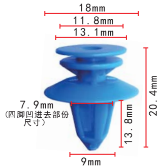
C961 POM Blue Trim Panel Retainer
