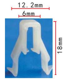
C1311 Nylon Original Trim Cover Clip Ford
