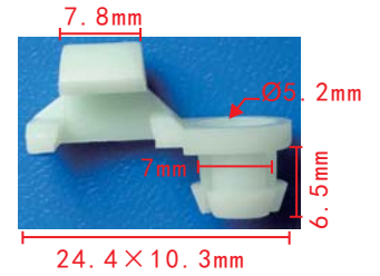
C616 Nylon Green Tailgate Rod Clip GM 14037239, 15545178
