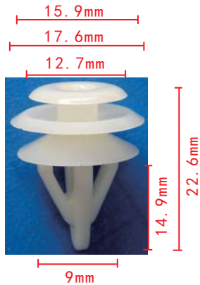
C64 Nylon White Trim Panel Retainer Honda 91566-SP0-003
