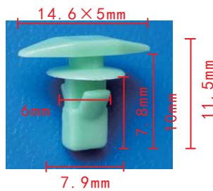
C628 POM Green Weatherstrip Retainer Honda 90664-671-0030 91568-SR2-003
