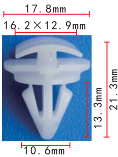
C1410 POM White Door Trim Panel Retainer
