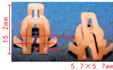
C1567 Nylon Orange GPS Inside Square Socket Retainer Suzuki
