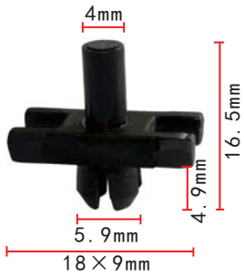
C234 Nylon Black Windshield Retaining Clip
