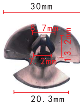
C1021 Nylon Black Hood Insulation Retainer Chrysler 4878883AA
