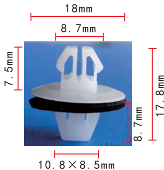
C378 POM White Rocker Panel Moulding Clip Toyota 90467-11063 Previa 1990-On
