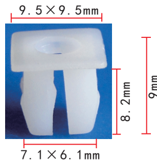
C418 POM White Headlight Adjusting Nut GM 1962-On 343543, 343555, 354076, 362379
