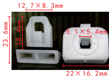
C1670 POM White Front Bumper Retainer Lexus 52197-30040
