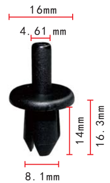
C678 Nylon Black Rocker Panel Push-Type Retainer Volvo 9133417-7
