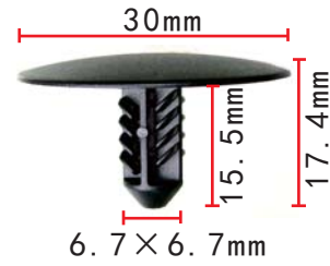
C3175 Nylon Black Engine Cover Heat Shield Clip GM#11571159
