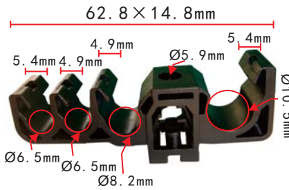
C1013 POM Black Routing Clip Toyota Hiace
