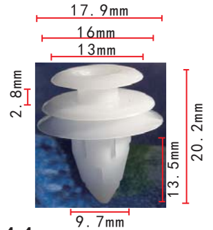
C244 POM White Trim Panel Retainer
