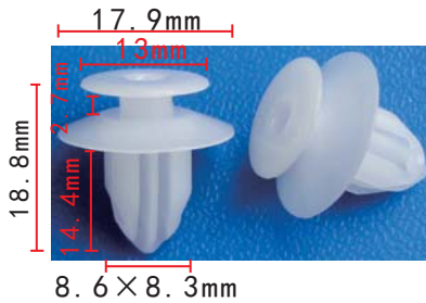
C1598 POM White Door Panel Retainer Honda
