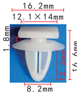
C935 Nylon Original Trim Panel Retainer
