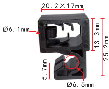
C1009 POM Black Routing Clip Toyota Hiace
