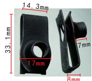
H2122 Zinc Black M8-1.25 Screw GM, Ford
