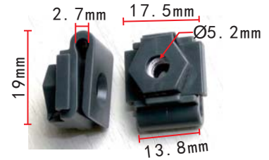
C3030 POM Dark Grey Bumper Retainer Nut Mazda
