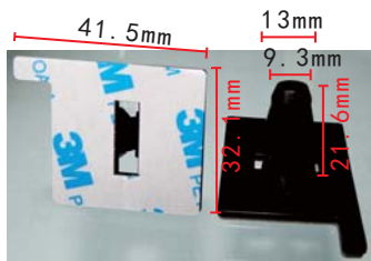
C1374 POM Black Windshield Retainer Square Bottom With 3M Adhesive Toyota Alphard
