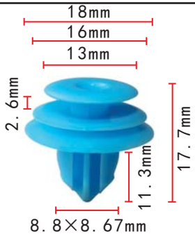
C256 POM Blue Garnish Moulding Retainer GM 88970345, Toyota 90467-10167 Nissan 76882-WA000
