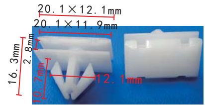
C1606 POM White Door Moulding Clip GM 15127746 Buick Terraza, Chevrolet Uplander, Pontiac Montana sv6, Saturn Relay 2005-On
