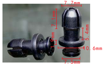
C1082 Nylon Black Push-Type Retainer
