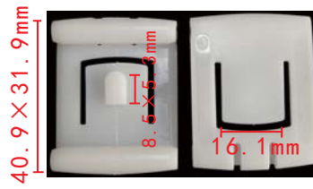
C1566 POM White Seat Slide Block VW Jetta
