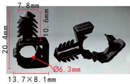
C1813 Nylon Black Hole Tube Retaining Clip
