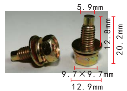
H2110 Zinc Color Screw
