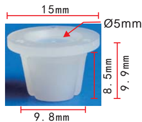
C972 Nylon White Headlight Assembly Grommet Hyundai 92351-37000
