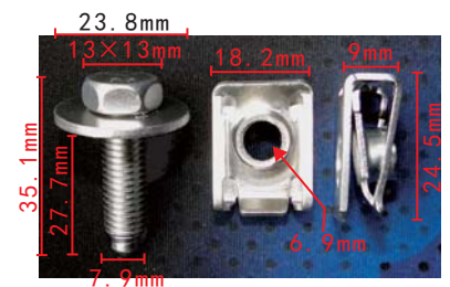
H2098 Zinc Silver Iron Clip & Screw Audi, Mercedes-Benz
