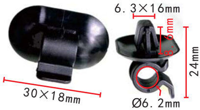
C3069 Nylon Black Engine Cover Poles Base Clip Peugeot#792834
