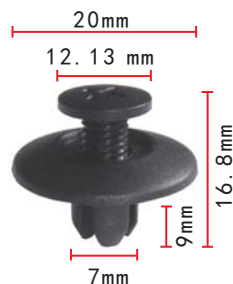
C92 Nylon Black Push-Type Retainer T-100 1992-On 90467-07044
