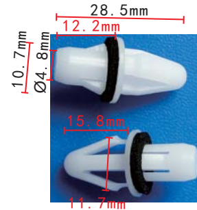
C1439 POM White Retainer Nissan 85099-AU000
