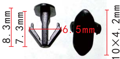
C1997 Nylon Black Rear Door Sealing Strip Clip Honda#90651-T2M-003
