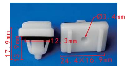
C1958 POM White Rocker Panel Sill Fender Clip Hyundai#87758-2S000
