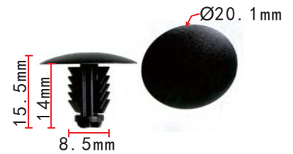
C3017 Nylon Black Rear Frame Trim Panel Retaining Clip Fiat#0735266957,1RZ74JXWAA
