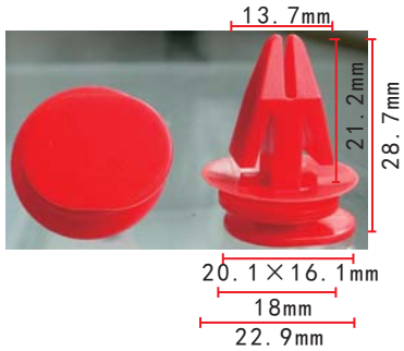
C1561 POM Red Lower Side Sill Retainer
