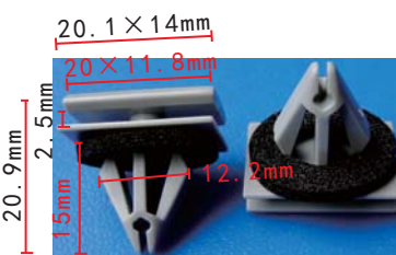
C1604 POM White Rocker Panel Retainer
