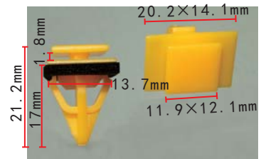
C1956 POM Yellow Rocker Panel Sill Fender Clip Hyundai#87759-3V000
