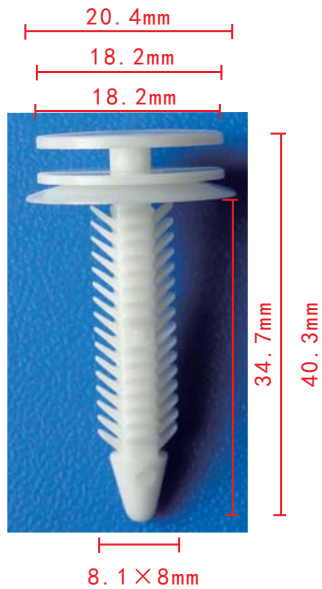
C687 Nylon White Door Trim Panel Retainer GM 1997-On 10421018
