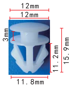
C1298 POM White Fender Trim Retainer VW 191853585A; Audi
