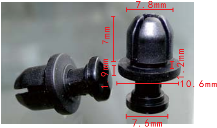
C1078 Nylon Black Push-Type Retainer
