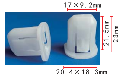
C1440 POM White Glove Compartment Retainer Toyota 90467-14023
