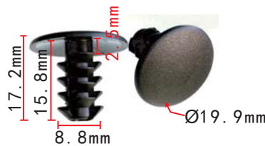
C3005 Nylon Black Retaining Clip Fiat#0718115080,68095492AA
