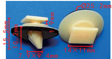
C3205 POM Yellow Door Trim Panel/Rear Spoiler Retaining Clip Mazda#KB8A-51-SJ3
