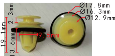
C1949 POM Yellow Door Trim Panel Retaining Clip Honda#91560-TX4-A01
