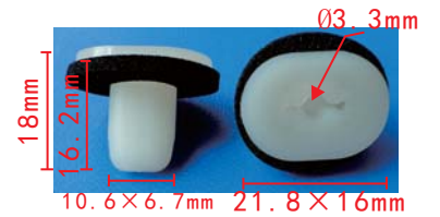
C1521 Nylon Original Screw Mazda
