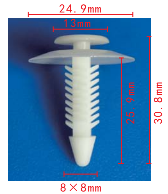
C591 Nylon Natural Trim Panel Retainer GM 10158124
