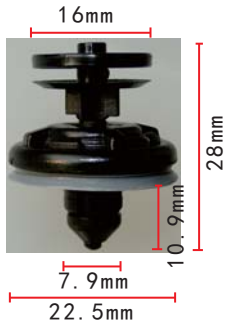
C1250 Nylon Black Door Trim Panel Retainer
