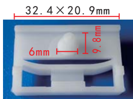
C1482 POM White Body Side Sill Fastener BMW 51718184574
