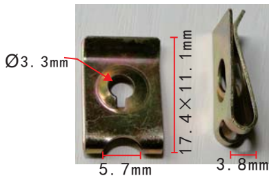
H2101 Zinc Color U-Type Iron Clip
