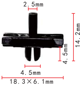
C234 Nylon Black Windshield Retaining Clip
