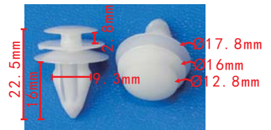
C3222 POM White Tail Gate/Trunk Liner Trim Panel Retainer
