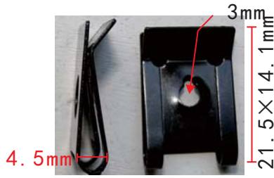
H2129 Zinc Black Iron Clip
