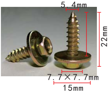
H2123 Zinc Color Screw
