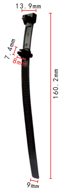
C233 Nylon Black Cable Strap Mercedes-Benz 114-997-02-90
