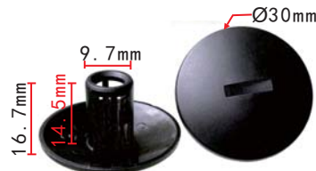
C1913 Nylon Black Wheel Arch Retaining Clip RENAULT#7703081227
