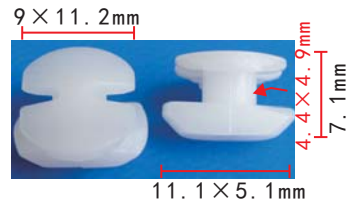
C1381 POM White Retainer Mercedes-Benz W202, W210, W220
