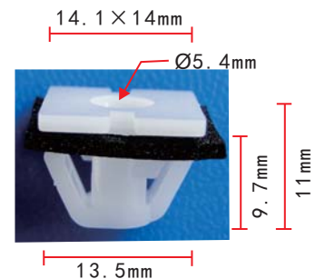
C365 POM White Body Side Moulding Clip With Sealer #8 Screw Size
