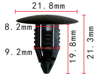
C1257 POM Black / Grey Retainer
