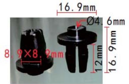
C1826 Nylon Black Retaining Nut Toyota 90189-05144
