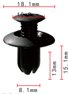
C578 Nylon Black Push-Type Retainer Mazda; Ford Rocker Panel Trim Panel Retainer Hyundai
