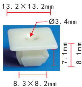
C27 Nylon Beige Grille Nut #8 or #10 Screw Size
