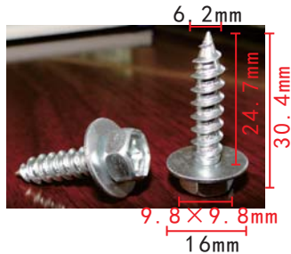
H2131 Zinc Silver Bolt Toyota 90159-60488
