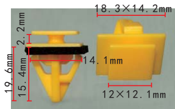
C1957 POM Yellow Rocker Panel Sill Clip Hyundai#87756-3N100
