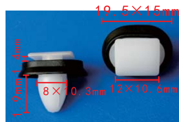
C1762 POM Origin Trim Strip Retaining Clip Fiat 71728806 ; Citroën 856543
