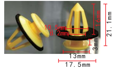
C1557 Nylon Yellow Door Trim Panel Retainer Jaguar
