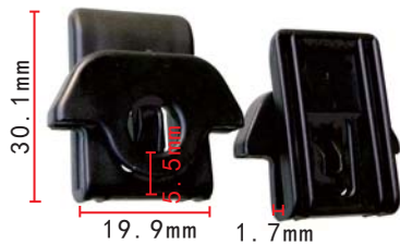
C1991 Nylon Black Wheel Arch Fender Fixed "U" Nut Nissan#63848-9Y000
