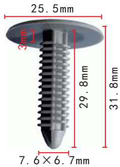
C990 Nylon Grey Headliner Retainer GM 15006827
