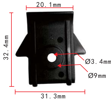
C814 Nylon Black Fender "U" Nut #10 Screw Size Panel Thickness: 2mm Nissan 63848-35F00
