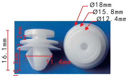
C1656 POM White Door Panel Retainer Land Rover LR028939
