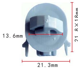
C983 Nylon Light Blue Rocker Panel Moulding Clip Nissan Loulan, Murano 2003-On
