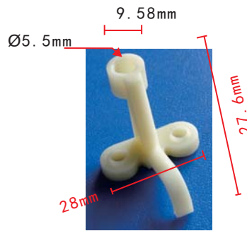
C311 Nylon Beige Headlight Adjusting Screw & Nut Assembly GM 5949838 Chevrolet, Buick & Pontiac
