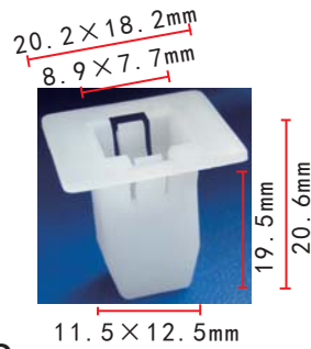
C238 Nylon White Bumper Grommet
