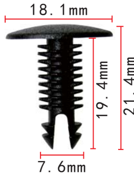
C1255 Nylon Black Retainer
