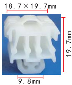
C920 POM White Retainer Mercedes-Benz
