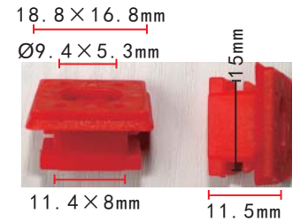
C1487 Nylon Red Hardware insert Door Trim Panel Retainer BMW 51458266814
