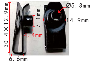
H2121 Zinc Black Iron Clip
