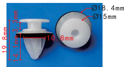
C1976 POM Original Fender Flare Moulding Clip Mazda#KD51-51-W24
