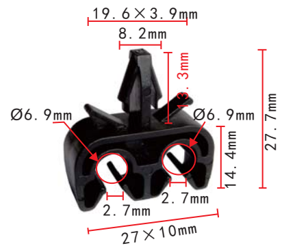
C1015 POM Black Routing Clip Toyota Hiace
