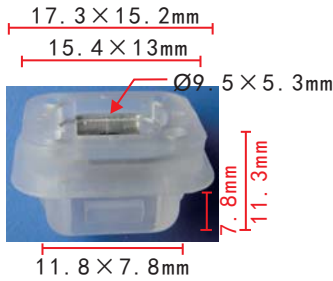
C1432 Nylon Original Door Trim Panel Retainer
