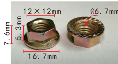
H2115 Zinc Color Nut
