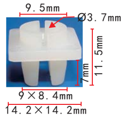
C1390 Nylon White Nut Toyota
