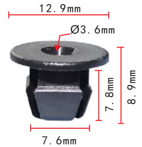
C137 Nylon Black Tail Light Nut #8 Screw Size
