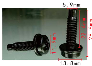
H2117 Zinc Black Screw
