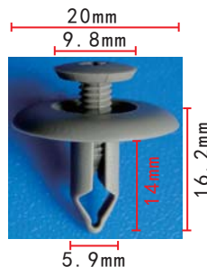
C1449 Nylon Coffee Push-Typer Retainer Mazda B042-68-865 05; Honda
