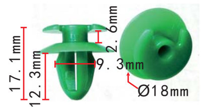
C3174 POM Green Door liner/Speaker System Retaining Clip BMW#51411870718
