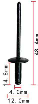
H2012 Auto Aluminum Rivet Toyota 90269-06054
