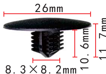
C3167 Nylon Black Engine Cover Heat Shield Clip Mitsubishi#MU001282
