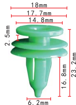
C977 POM Green Door Trim Retainer Chrysler, Lexus
