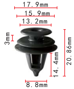
C270 Nylon Grey Trim Panel Retainer
