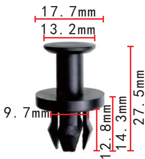
C3188 POM Black Rear Bumper Retainer VW#WHT-005-263
