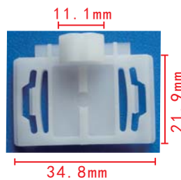
C912 POM White Lower Side Sill Rocker Panel Retainer VW & Audi
