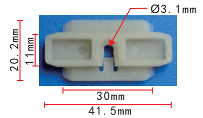
C927 Nylon Green Anti-Dust Clip VW
