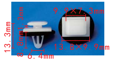
C1970 POM White Window Frame Retaining Clip 8235A1431
