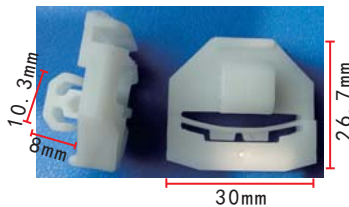
C1305 POM White Retainer European Car
