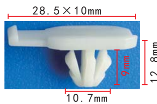
C972 Nylon White Headlight Assembly Grommet Hyundai 92351-37000
