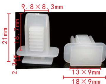
C1653 Nylon Original Retainer Land Rover L63808
