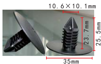
C1556 Nylon Black Hood Insulation Panel/ Hood Insulation Cotton Retainer Mercedes-Benz Renault 7703077435
