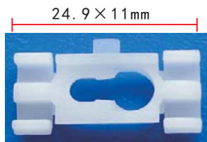
C437 POM White Moulding Clip
