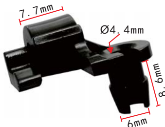
C324 Nylon Black Door Lock Rod Clip Used On Left-Hand Side GM 1971-On 19815325, 16607593 Ford 1972-On D2VZ-6521952A7
