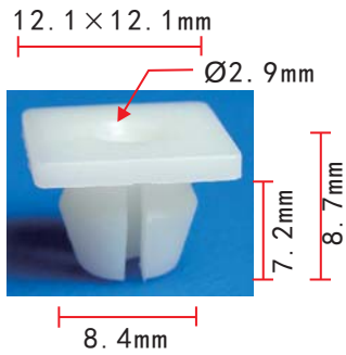
C28 Nylon White Headlight Bezel Nut #8 Screw Size GM 14013246
