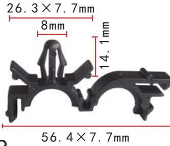
C52 Nylon Black Routing Clips for Wire Loom Inside Diameter: \Phi 14.3\text{mm} GM 8911472
