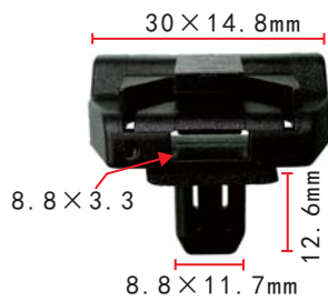
C1479 Nylon Black Retainer Toyota Highlander
