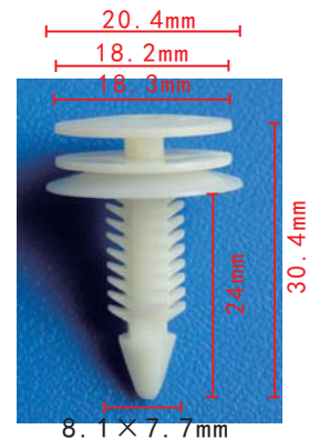
C635 Nylon Natural Trim Panel Retainer GM 10285935
