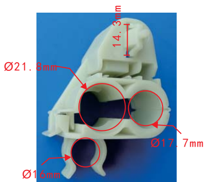
C1492 POM White Bumper Retainer Toyota Lexus Toyota Estima MCV40 2000-2003 On
