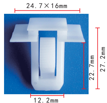
C416 POM White Windshield to Panel (Lower) Side Moulding Clip GM 1975-On 9731301 AMC 1975-On 4005540
