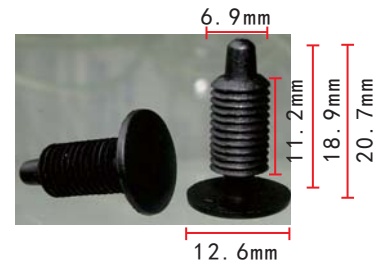
C1618 Nylon Black Trim Panel Retainer GM
