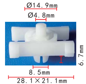
C1488 POM White Body Moulding Retainer BMW 51131829904
