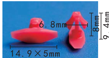
C1965 POM Rose Red Rocker Panel Sill Fender Clip Hyundai#87756-2W000
