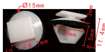
C1656 POM White Door Panel Retainer Land Rover LR028939
