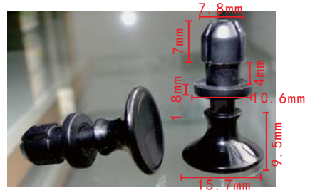
C1081 Nylon Black Push-Type Retainer
