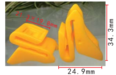
C1631 POM Yellow Rear Bumper Retainer Nissan
