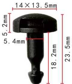
C1469 Nylon Black Retainer Nissan 01553-04463
