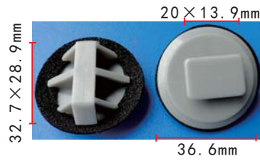
C1516 POM Grey Sealing Clip Mazda
