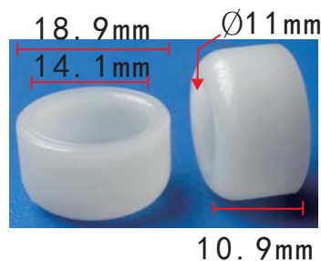
C1629 Nylon White Japanese Car
