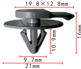
C1436 POM Grey Wheel Trim Retainer
