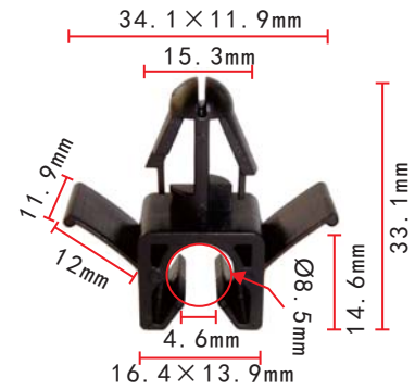
C1016 POM Black Routing Clip Toyota Hiace
