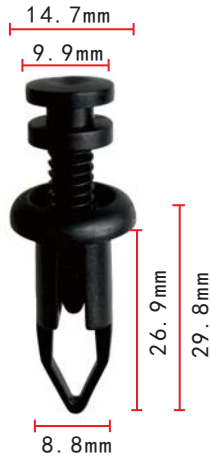
C189 POM Black Push-Type Retainer Nissan; Toyota; Suzuki; Mitsubishi
