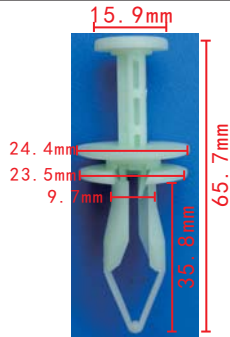
C1663 Nylon Light Green GM 10426555
