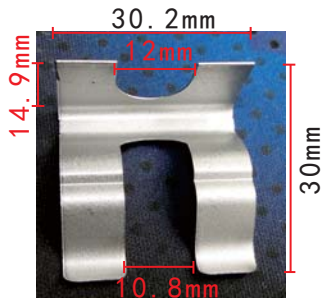
H2148 Zinc Silver Iron Sheet Toyota
