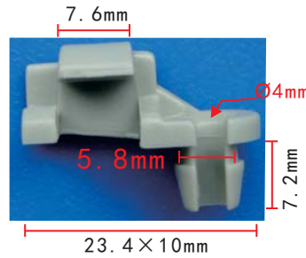
C185 Nylon Beige Push-pull Rod, Door Lock Rod & Engine Rod Clip
