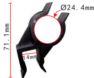
C1367 Nylon Black Engine Routing Clip Toyota Alphard
