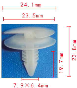
C20 Nylon Beige Rear Quarter Panel Retainer GM 20480475
