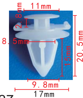
C1527 POM White Trim Panel Retainer Mitsubishi MR200275
