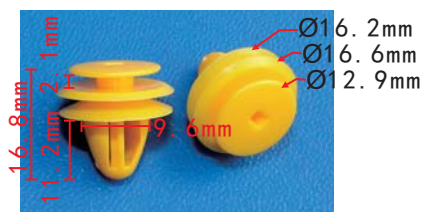
C1995 POM Yellow Door Trim Panel Retaining Clip Hyundai#82315-38000
