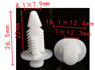
C1658 POM White Rocker Panel Retainer
