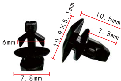
C1472 Nylon Black Body Weather Strip Retainer Honda 91530-S0A-003
