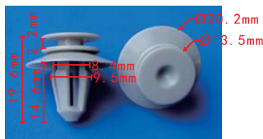
C1953 Nylon Grey Roof Liner/ Door Trim Clip Mercedes#A0089880978
