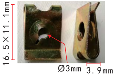
H2100 Zinc Color U-Type Nut
