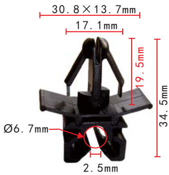
C1011 POM Black Routing Clip Toyota Hiace
