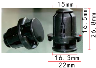
C1564 POM Black Side Sill Clip / Suspension Cover Retainer / Apron Clip
