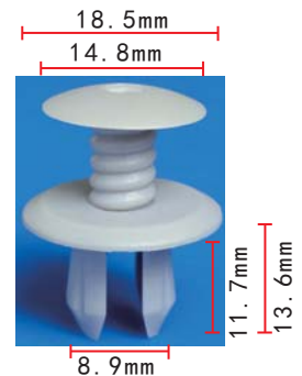
C929 Nylon Grey Door Trim Panel Retainer VW 701867299
