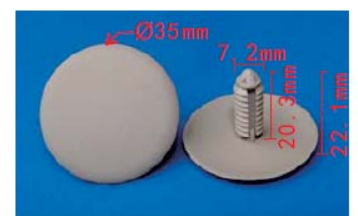
C1838 Nylon Light Grey Car Roof / Sun Visor Retaining Clip Chrysler TY98TL2-AA
