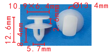
C3190 POM White Mirror Inner Trim Triangle Retaining Clip VW#6E0-837-732
