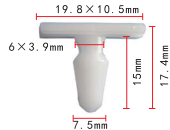
C975 POM White Retainer Peugeot
