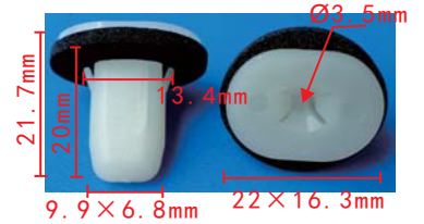
C1521 Nylon Original Screw Mazda
