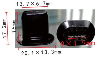
C1578 Nylon Black Retainer Peugeot, Renault
