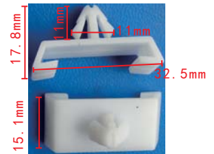
C1572 POM White Door Outer Trim Panel Retainer VW 330-853-858
