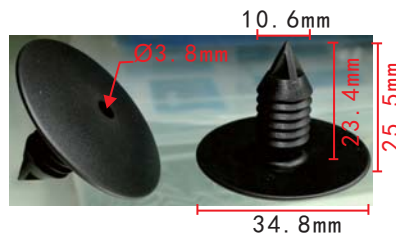
C1520 Nylon Black Engine Cover Insulation Retainer Renault
