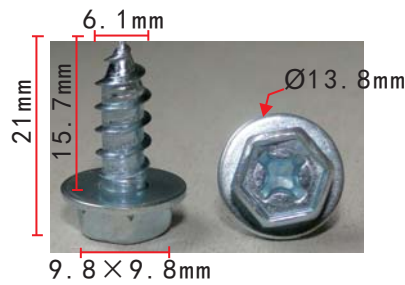
H2152 Zinc Blue Hexagon Tapping Screw Toyota 90159-60303
