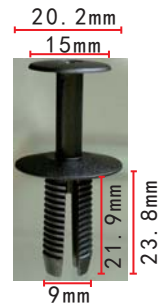
C1533 Nylon Black Fender Lining Retainer BMW 51127004445
