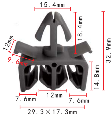
C1012 Nylon Grey Routing Clip Toyota Hiace
