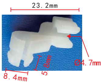
C349 Nylon White Door Lock Rod Clip-Right
