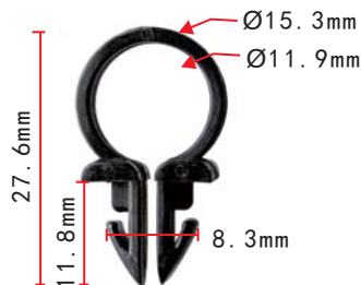
C498 Nylon Black Routing Clips for Wire Loom
