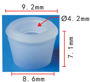
C897 Nylon White Moulding Insert Mercedes-Benz 000-987-10-81
