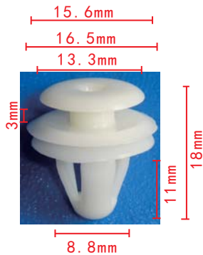
C67 Nylon Original Door Trim Panel & Garnish Retainer Toyota ; Subaru ; Mitsubishi
