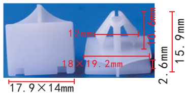
C1624 POM White Rocker Panel Retainer GM 15236894 Buick Lucerne, Cadillac CTS & STS 2003-On
