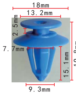
C960 POM Blue Trim Panel Retainer
