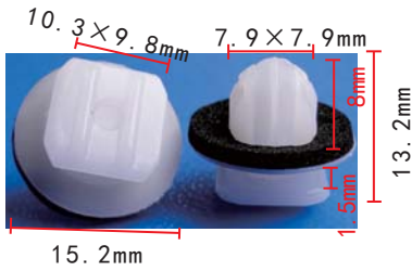
C1598 POM White Door Panel Retainer Honda
