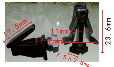
C1632 POM Black Bumper / Grille Retainer Nissan
