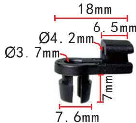
C3210 Nylon Black Door Lock Rod Clip
