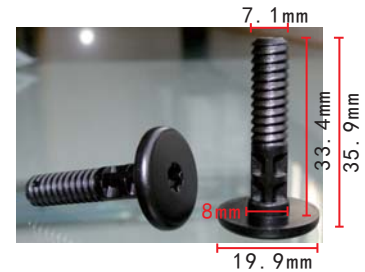
C1558 POM Black Lower Side Sill Rivet/ Rocker Trim Panel Retainer BMW Series 1/3/6/X1/X6
