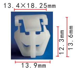
C295 POM White Body Side Moulding Clip
