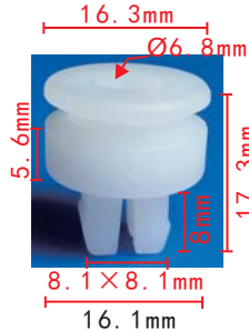
C1530 Nylon White Screw Seat Subaru 94019FA070
