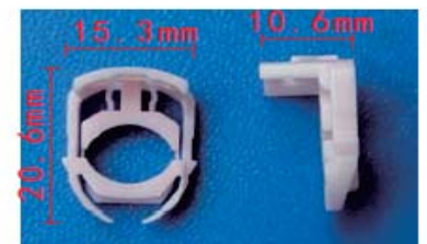
C1837 POM Pink Fuel Line Retainer Clip Ford 7L3Z-9S317-A
