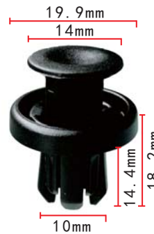
C1518 POM Black Bumper Retainer Honda Acura
