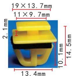
C969 POM Yellow Rocker Moulding Clip With Sealer Hyundai 87758-35000 Accent, Santa Fe & Tiburon 1995-On
