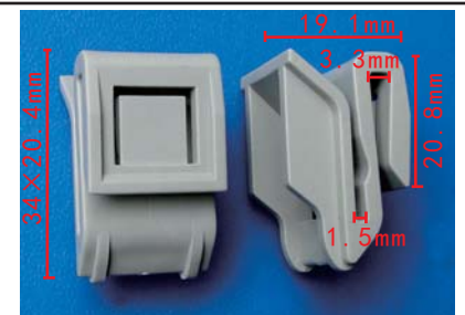
C3229 POM Grey Rear Bumper Bracket Nissan#85284-JD00A
