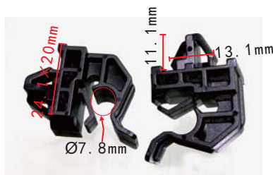
C1960 Nylon Black Hood Prop rod Retaining Clip Hyundai#81174-2L000
