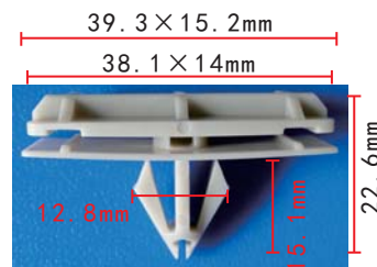
C1484 POM Grey Rocker Panel Clip Jeep Liberty
