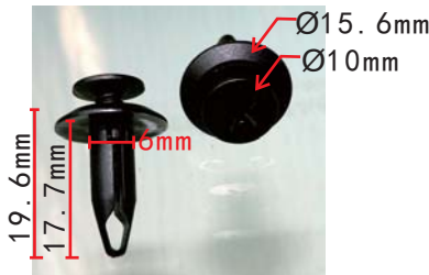
C1733 Nylon Black Wheel Trim / Radiator Bracket Retaining Clip Mercedes-Benz A000-991-63-98
