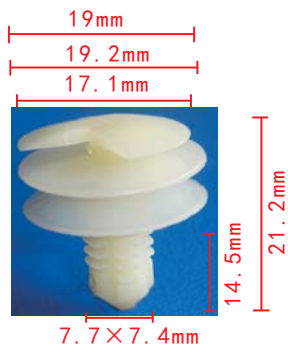
C12 Nylon Beige Door Trim Panel & Roof Liner Retainer GM 1971-78 3065575, 2064891, 9818648, 9883583
