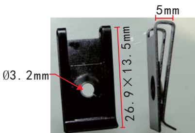
H2128 Zinc Black Iron Clip
