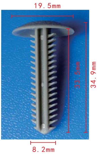
C600 Nylon Grey Door Trim Panel Retainer Chev. Astro & GMC Safari Mini Vans 1994-On 15986343
