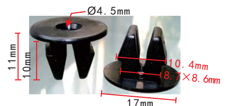
C1609 Nylon Black Fender Nut Toyota Lexus 90189-06211
