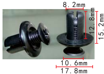
C1542 Nylon Black Wiper Cover Retainer
