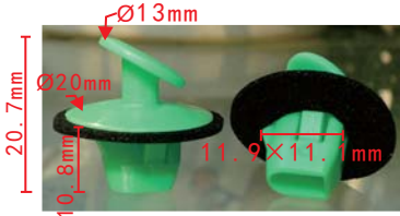
C1664 POM Green Inner Trim Panel Retainer Lexus 81496-50010
